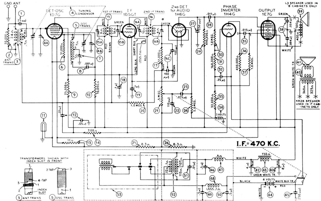
Fig. 4. Schematic Diagram—Model 38-34, Code 125
