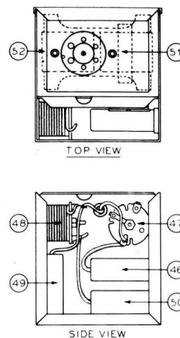
Fig. 5. Vibrator Part Locations
