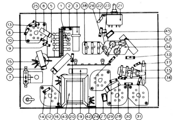
Fig. 6. Part Locations Underside of Chassis
